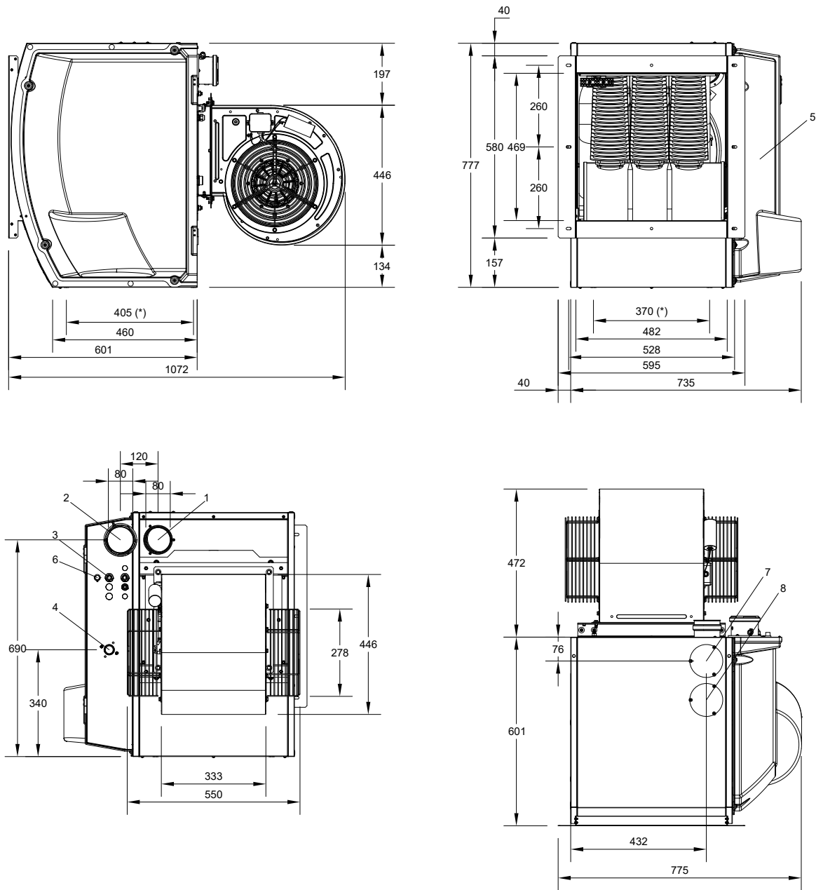
Figure 4.8 Unit dimensions
