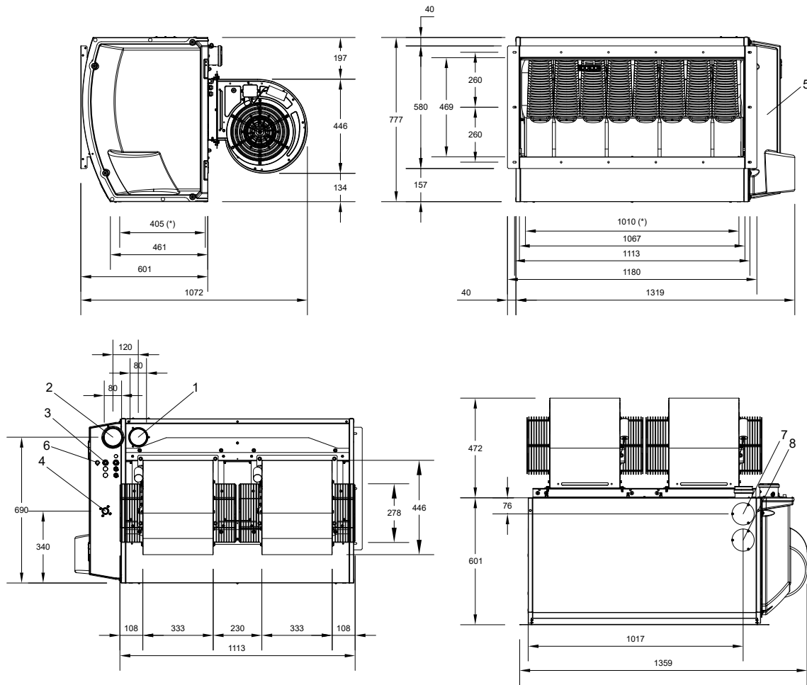
Figure 4.10 Unit dimensions
