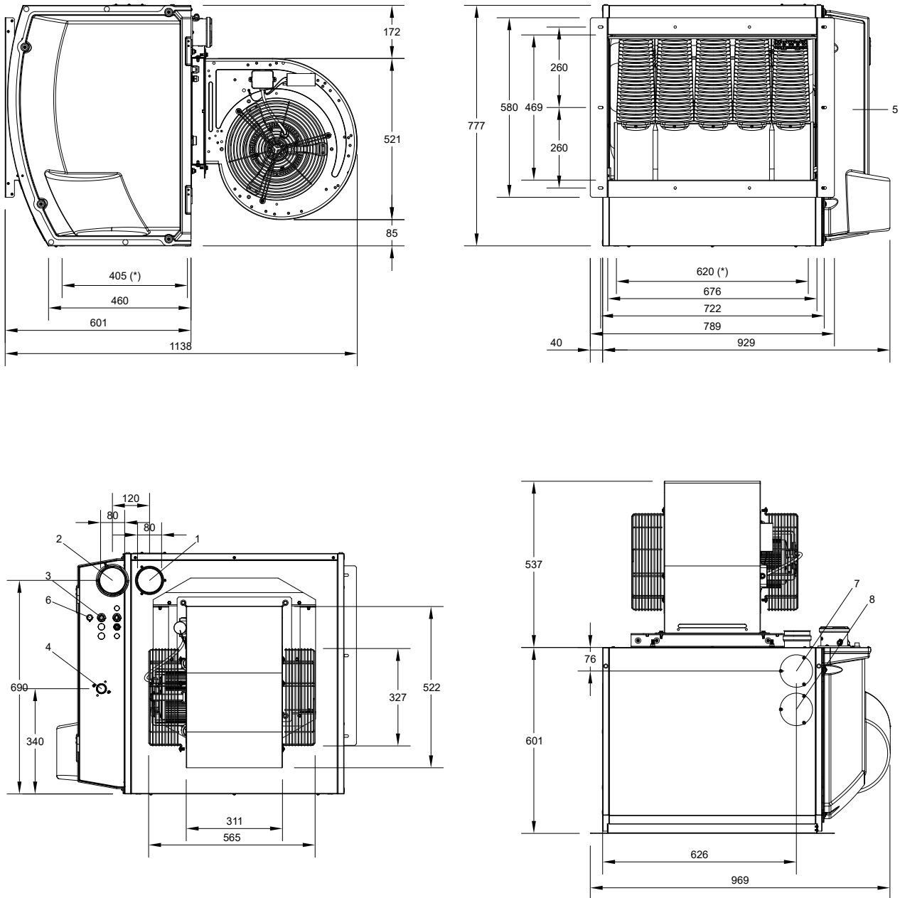
Figure 4.9 Unit dimensions
