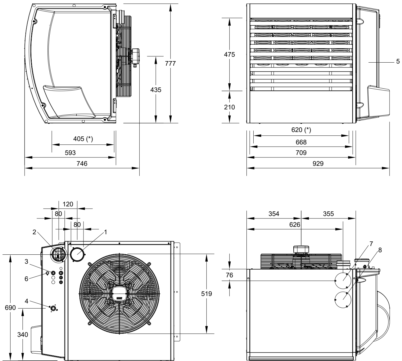
Figure 4.4 Unit dimensions
