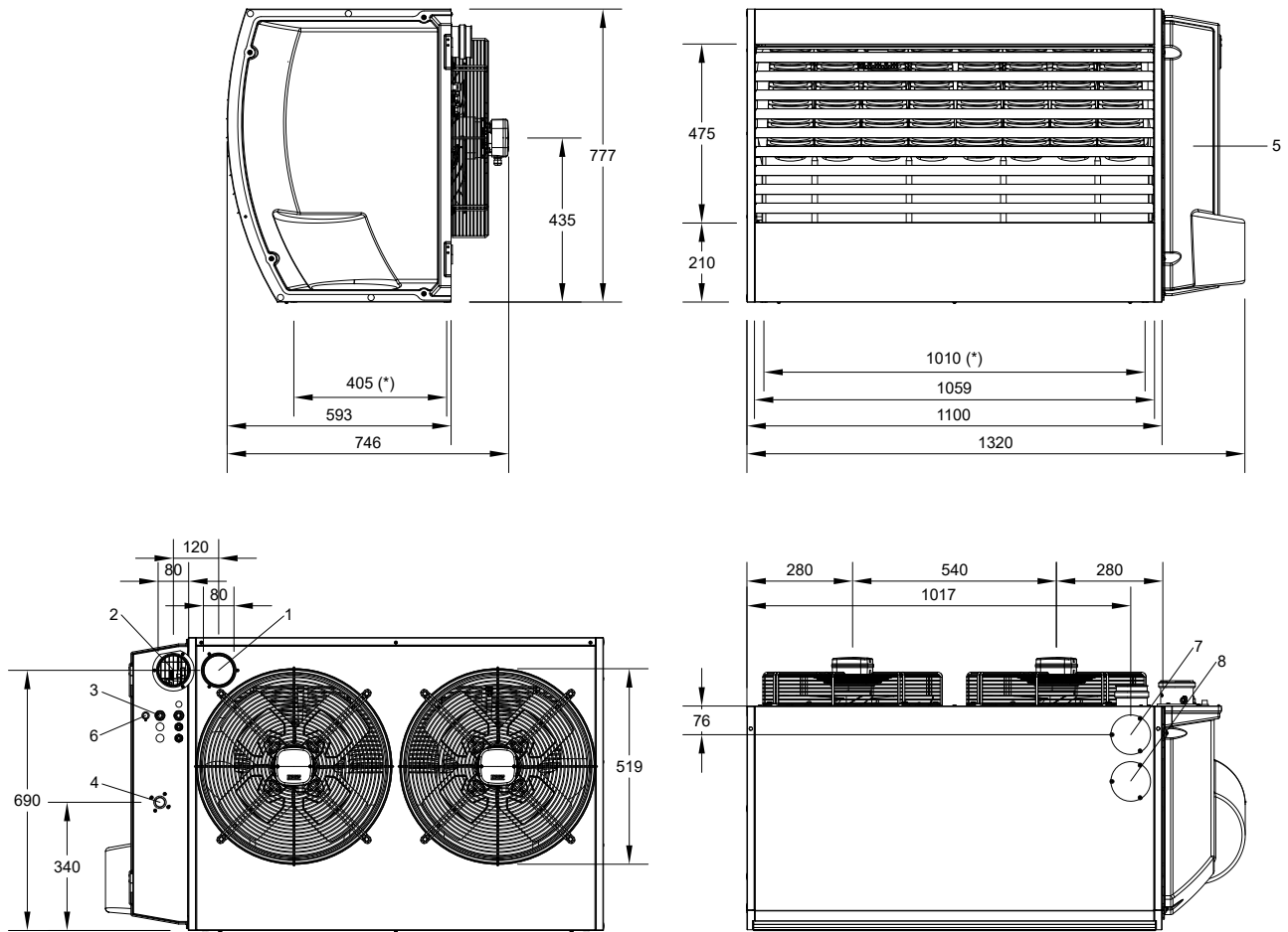
Figure 4.6 Unit dimensions
